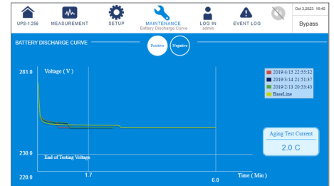
Battery discharging curve
